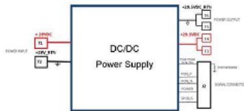
Block Diagram of the 1700W Power Supply
